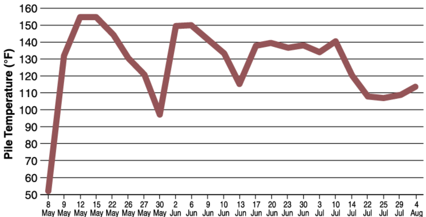
Figure 3. Average temperatures of a strawbedded beef feedlot manure compost pile. The manure was piled into windrows on May 8. The pile was turned on May 30, June 13,
